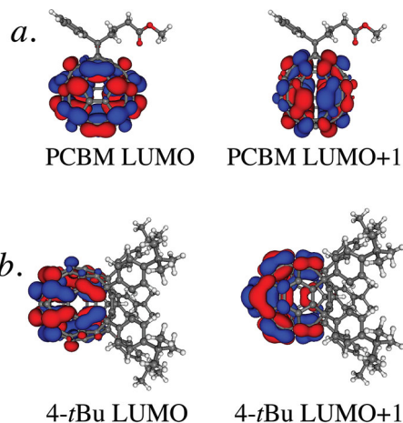
Figure 2. Kohn-Sham orbitals from our DFT calculations corresponding to the LUMO and LUMO+1 of the isolated fullerene molecules: a) PCBM, and b) 4- t Bu. The orbitals were calculated using the B3LYP functional and STO-3G basis set (see SI for details).
