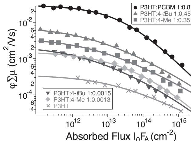
Figure 3. The dependence of \varphi \Sigma \mu , calculated from the measured TRMC photoconductance via Equation 1, on absorbed photon flux ( I_0 F_A ) for pure P3HT and blends with different fullerenes. The solid curves are fits to Equation S3 in the SI.
