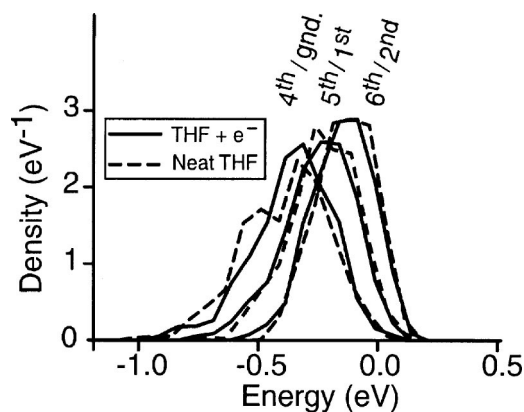
FIG. 5. Comparison between the normalized distributions of energy for the equilibrated THF-solvated electron eigenstates (solid curves) and for the eigenstates of an excess electron injected into neat THF (dashed curves). The energy probability distributions in the neat liquid were calculated from an 8 ps trajectory, whereas the distributions for the solvated electron were calculated from the full 32.5 ps equilibrium trajectory.
