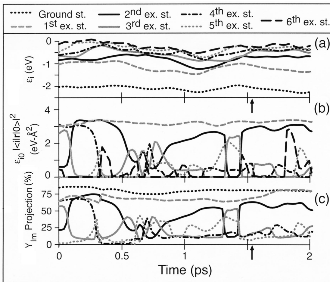
FIG. 2. Time dependence of (a) the eigenvalues, (b) the transition dipole moments, and (c) the spherical harmonic projections of the lowest six eigenstates of the THF-solvated electron shown over a small window in the middle of our 32.5 ps equilibrium trajectory. The key for panel (b) should be read as the transition from the ground state (labeled as 0) to the i th excited state; \epsilon_i is the energy of state i and \epsilon_{i0} is the energy gap between the ground state and the i th state. The projection (see the Appendix and Ref. 58) of each excited eigenfunction onto the l=1 ( p -like) spherical harmonic is shown, as is the projection of the ground state onto the l=0 ( s -like) spherical harmonic. The spherical harmonic projection of the sixth excited state is not shown in panel (c) because this state has no significant spherical symmetry. The arrows indicate the specific configuration examined in Fig. 4.
