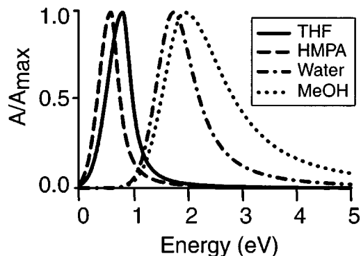
FIG. 1. Gaussian-Lorentzian fits to the experimental absorption spectra of the solvated electron in THF (solid curve), HMPA (dashed curve), water (dash-dot curve), and methanol (dotted curve). The fitting parameters were taken from Ref. 12.
