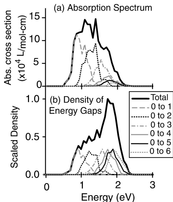
FIG. 3. (a) Calculated absorption spectrum for an excess electron in THF using Eq. (3). Underlying the total spectrum (thick black curve) are the individual transitions from the ground to each of the excited states (thin gray and black curves). (b) The scaled density of energy gaps of the THF-solvated electron between the ground and each of the six lowest excited states, defined as the distribution of instantaneous energy gaps between the ground and each of the excited states.
