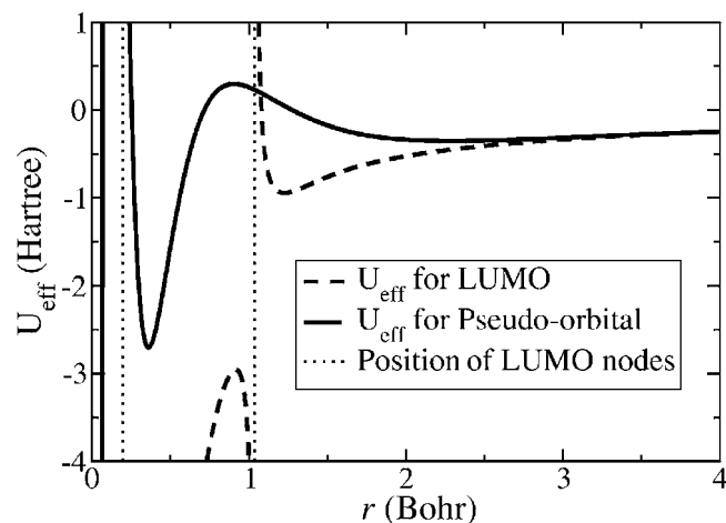
FIG. 3. Kinetic-energy-minimized PK effective potential for the valence electron/Na + interaction. The dashed curve shows the effective potential for the LUMO calculated via Eq. (20) for |\phi\rangle=|\psi_{3s}\rangle (the orbital displayed as a dashed curve in Fig. 1); i.e., this curve is the Na + LUMO HF potential, which for clarity is shown only for r>0.5 a.u. The vertical dotted lines indicate singularities in the LUMO HF potential (where the LUMO has radial nodes). The kinetic-energy-minimized PK effective potential, which has no singularities, is shown by the solid curve.
