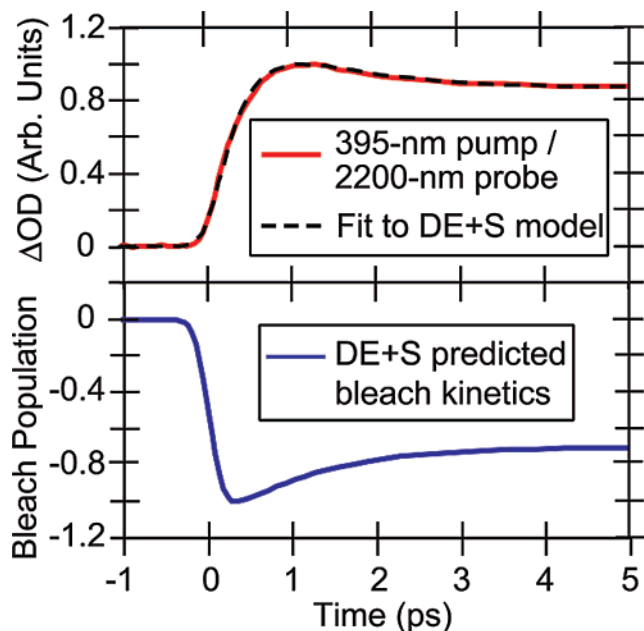
Figure 4. Upper panel: The 2200-nm transient absorption dynamics following the 395-nm CTTS excitation of \text{Na}^- in THF (red solid curve) and a fit to this data to the DE/DE+S model (black dashed curve; see the Appendix and ref 26 for details of the models). Lower panel: The predicted \text{Na}^- bleach dynamics derived from the DE/DE+S model based on the parameters obtained from the fit to the electron data in the upper panel.
