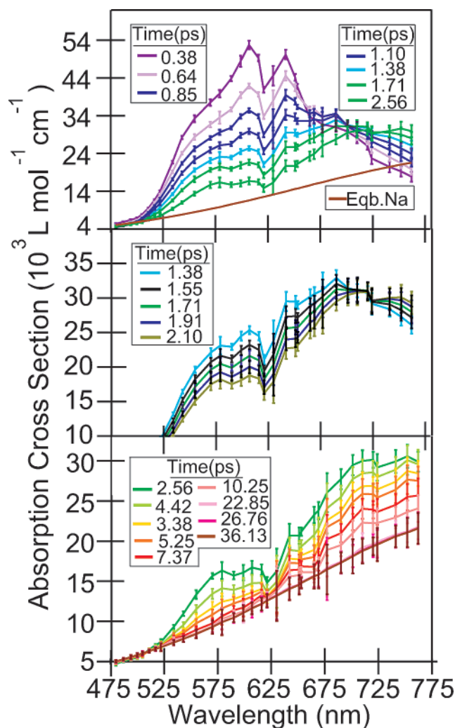
Figure 6. Reconstructed transient spectra of the neutral sodium species created following 395-nm CTTS excitation of Na - in THF from Figure 5, but scaled by the population dynamics, which was assumed by stoichiometry to be the same as the dynamics of the Na - bleach in the lower panel of Figure 4. The upper panel shows the early time dynamics associated with the solvation of the weakly-solvated sodium atom. The lower panel shows the long-time dynamics characteristic of the slow solvation of the newly-formed contact pair to form the well-known equilibrium species whose absorption spectrum is shown as the green dashed curve in Figure 1. The center panel presents the dynamics from 1.38 ps to 2.1 ps on an expanded scale, where a clear isosbestic point can be observed near 720 nm. The isosbestic point is a clear sign of a chemical reaction, which we assign as the conversion of the solvated sodium atom into an unsolvated atom (Na + ,e - ).
