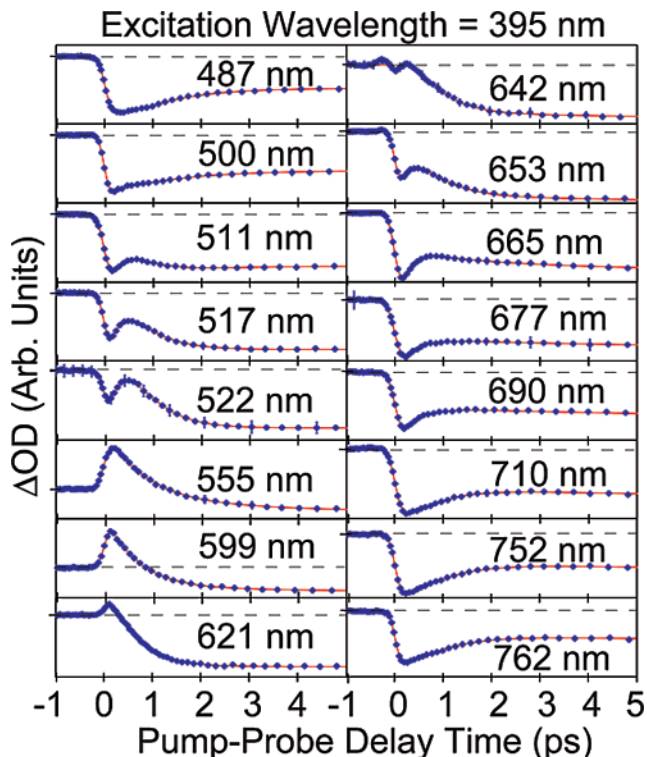
Figure 3. Selected subset of the 33 pump-probe transients collected for the 395-nm CTTS excitation of Na - in THF and probing at various wavelengths in the visible region, as indicated for each transient. The blue dotted curves are the normalized raw data, and the red solid curves are the fits of up to eight exponentials convoluted with the instrument response to provide an analytic representation of the data, as described in the text.
