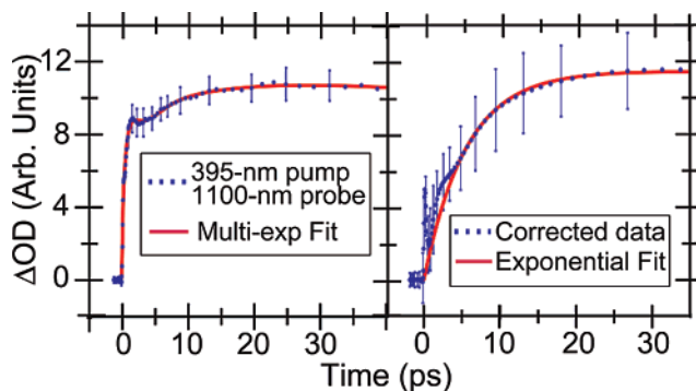
Figure 10. Left panel: Spectral transient probing at 1100 nm following the 395-nm CTTS excitation of Na - in THF (blue dots) and fit to eight exponentials convoluted with the instrument function to provide an analytic representation of the data (red curve, see text for details). A comparison to Figure 1 shows that the Na - bleach has no spectral contribution at this wavelength. Right panel: The same data as in the left panel, but with the spectral contribution from the solvated electron subtracted to reveal the dynamics of the neutral sodium species (blue dots). The electron's spectral kinetics were assumed to match those at the other IR wavelengths shown in Figure 2. The red curve in this panel is a fit to an exponential rise with a time constant of \sim 5.5 ps, reflecting the solvation dynamics of the tight sodium cation/electron contact pair. The poor fit at early times is likely due to absorption from the excited CTTS electron and a small amount of immediate contact-pair recombination that has not been accounted for in the analysis.
