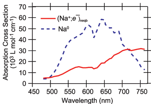
Figure 7. Spectra of the equilibrated weakly-solvated sodium atom (blue dashed curve) and the unsolvated tight sodium atom/electron contact pair (red solid curve) obtained from performing singular-valued-decomposition (SVD) modeling on the spectra in the center panel of Figure 6. See ref 62, the text, and Part 2 of the Supporting Information for more details on the SVD modeling used to obtain these spectra.
