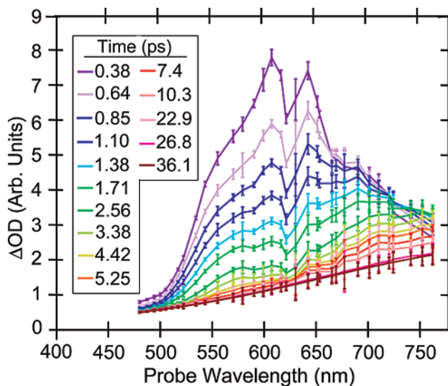
Figure 5. Transient spectra at representative times from 0.38 ps to 36.1 ps of the neutral sodium species formed following the 395-nm CTTS excitation of \text{Na}^- in THF. To obtain these spectra, the raw data (a subset of which is shown in Figure 3) were first scaled at t = 30 ps using the known equilibrium cross-sections of the \text{Na}^- bleach, solvated electron and neutral sodium species; see the text and Figure S1 of the Supporting Information for more detail on the treatment of the raw data. After forming the scaled transient spectra, the contributions of the electron and \text{Na}^- bleach were subtracted, assuming that neither the bleach nor the electron undergo any spectral shifting and that the dynamics of the populations of these two species are as given in Figure 4. Because of the way this figure was constructed, the spectrum at \sim 30 ps is forced to match that of the known equilibrated neutral sodium species (green solid curve of Figure 1; see text for details). The absorption cross-sections are in arbitrary units.
