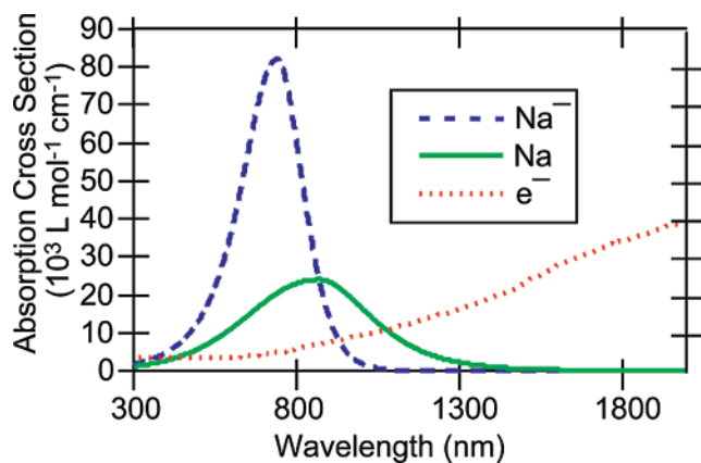
Figure 1. Equilibrium absorption spectra of the reactant and product species in the room-temperature CTTS reaction of \text{Na}^- in THF: \text{Na}^- (blue dashed curve, ref 21); the solvated electron (red dotted curve, ref 24); and the species whose stoichiometry is that of a neutral solvated sodium atom (green solid curve, ref 21). In this work, we assign the latter species as a (\text{Na}^+, e^-) contact pair with a high degree of atomic character.
