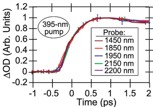
Figure 2. Transient absorption dynamics of the solvated electron produced following the 395-nm CTTS excitation of \text{Na}^- in THF. The electron's dynamics are probed at 1450 nm (dark-purple curve), 1850 nm (red curve), 1950 nm (blue curve), 2150 nm (green curve), and 2200 nm (light-purple curve). Each transient has been normalized at the maximum transient absorption to allow for better comparison of the dynamics at different wavelengths. The fact that the dynamics at all wavelengths are identical within the noise verifies that these traces reflect population dynamics of the ejected electrons and that there is no significant dynamic solvation of the electron following ejection.
