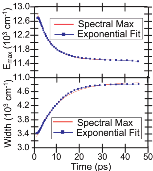
Figure 9. Energy maximum and width of the sodium cation/electron pair's spectra as a function of time after the 395-nm CTTS excitation of Na - , based on Lorentzian fits to the data in the lower panel of Figure 6 after subtracting the spectral contribution of the neutral sodium atom (whose spectrum and dynamics were obtained from the SVD analysis shown in Figure 7). The blue squares in the upper panel show the best-fit Lorentzian energy maxima, and those in the lower panel show the best-fit Lorentzian widths. The red curves are fits to single exponential functions with a best-fit decay time of \sim 5.9 ps for the energy maximum (upper panel) and \sim 9.7 ps for the spectral width (lower panel).
