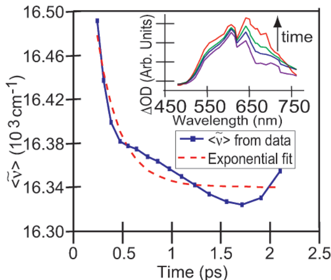
Figure 8. Average frequency of the weakly solvated neutral sodium atom's absorption spectrum as a function of time after the 395-nm CTTS excitation of \text{Na}^- , calculated using eq 2 from the spectra in the upper panel of Figure 6 after subtracting the spectral contribution from the tight sodium cation/electron contact pair (whose spectrum and dynamics were obtained from the SVD analysis shown in Figure 7). The average frequency data are shown as the blue squares, with the blue solid curve connecting the data points to guide the eye. The red dashed curve shows a fit to the data of a single exponential decay with a \sim 230 -fs time constant. The inset shows the representative corrected absorption spectra at a few select times: dark-blue curve, 240 fs; light-blue curve, 380 fs; green curve, 550 fs; red curve, 2100 fs.
