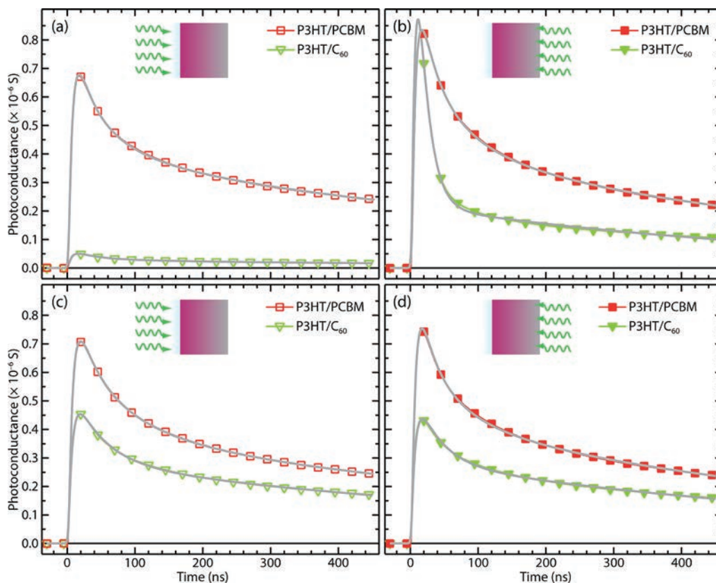
Figure 6. Photoconductance decay transients for sequentially deposited P3HT/fullerene samples, solution-deposited PCBM (red squares), and thermally evaporated C_{60} (green triangles), illuminated through the substrate (left) and through the fullerene overlayer (right): cartoons show the illumination geometry. The top panels show transients for the unannealed samples and the bottom panels for samples annealed at 150 °C for 20 min. The solid gray lines indicate fits to the data using eqs 4, 5, and 8.
