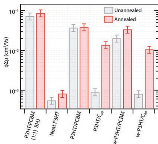
Figure 5. The product of the quantum yield ( \phi ) for mobile charge carrier generation and the sum of the mobilities ( \sum \mu ) for neat P3HT, a (1:1) P3HT:PCBM bulk heterojunction, and sequentially deposited polymer/fullerene layers with a combination of either solution-deposited PCBM or evaporated C 60 overlayers and P3HT or w-P3HT underlayers. Illumination was performed through the substrate at a wavelength of 500 nm.
