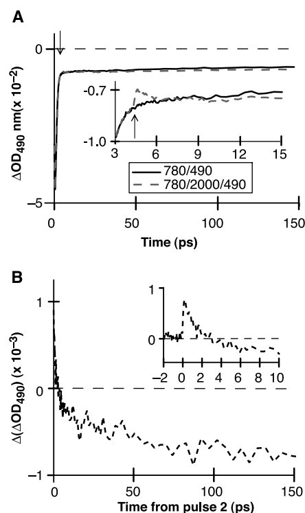
Fig. 3. (A) Comparison of a standard two-pulse experiment (780-nm pump, 490-nm probe, solid curve) with a three-pulse electron control experiment (780-nm pump, 2000-nm electron excitation, 490-nm probe, dashed curve) on \text{Na}^- in THF, with the electron excitation pulse arriving 4.4 ps after the 780-nm pump pulse so that recombination of immediate contact pairs is complete. (Inset) The same data near the arrival time of the 2000-nm electron excitation pulse on an expanded scale. The arrow marks the arrival time of the 2000-nm electron excitation pulse. (B) Dynamics induced by the 2000-nm excitation pulse [dashed curve; difference between the three- and two-pulse data shown in (A)]. (Inset) The same data on an expanded time scale.
