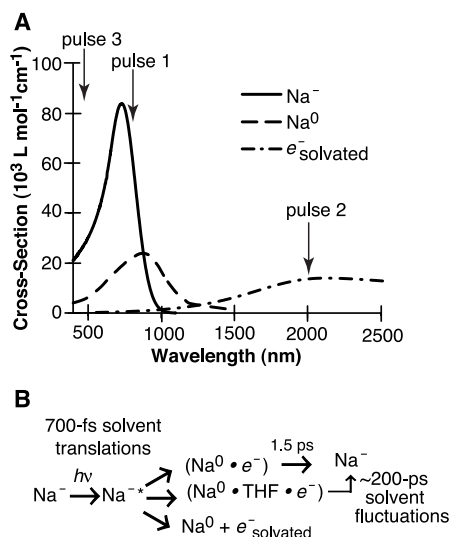
Fig. 1. (A) Steady-state absorption spectra of the major kinetic species in the CTTS reaction of sodide (Na - ) in THF: ground-state Na - [solid curve (5, 10)], the solvated neutral sodium atom [dashed curve (12, 13)], and the solvated electron [dot-dashed curve (11)]. The arrows show the spectral positions of the femtosecond light pulses used in the experiments. (B) A simplified kinetic scheme for the CTTS transition of Na - in THF based on (5–7); a more detailed scheme would also include the possibility of dissociation of the immediate and solvent-separated contact pairs. The branching ratio between immediate contact pairs, solvent-separated contact pairs, and free solvated sodium atoms-solvated electrons is determined by the wavelength of the CTTS excitation pulse.
