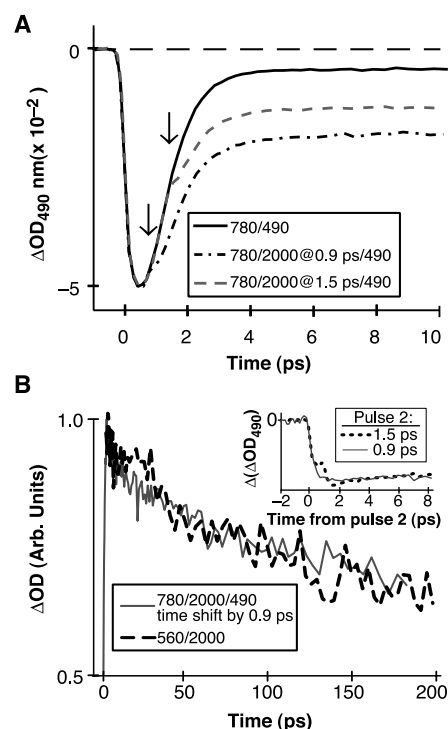
Fig. 2. (A) Comparison of a standard two-pulse experiment (780-nm pump, 490-nm probe; solid curve) with a three-pulse electron control experiment (780-nm pump, 2000-nm electron control excitation, 490-nm probe) on Na - in THF, with the electron excitation pulse arriving during the recombination of immediate contact pairs, either 0.9 ps (dot-dashed curve) or 1.5 ps (dashed curve) after the 780-nm pump pulse. The arrows indicate the arrival time of the 2000-nm electron excitation pulse. (B) Comparison of the three-pulse experiment [thin solid curve; same as dashed curve from (A) with the zero of time shifted to coincide with the 2000-nm reexcitation pulse] with a two-pulse experiment in which Na - is excited near 560 nm and the recombination dynamics are probed at 2000 nm (dashed curve); the curves have been arbitrarily scaled for better comparison. (Inset) The short-time dynamics of the difference between the two- and three-pulse signals shown in (A) (thin solid curve for 0.9-ps delay, dotted curve for 1.5-ps delay); these two curves have been scaled to the same maximum for better comparison.
